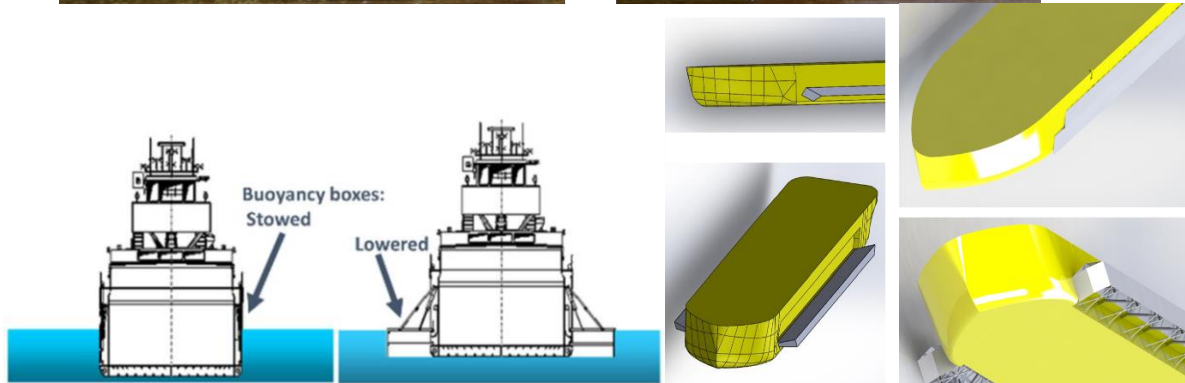
Figure 22: First concept of added buoyancy suitable for newbuilts and retrofits (source: Novimove project)
