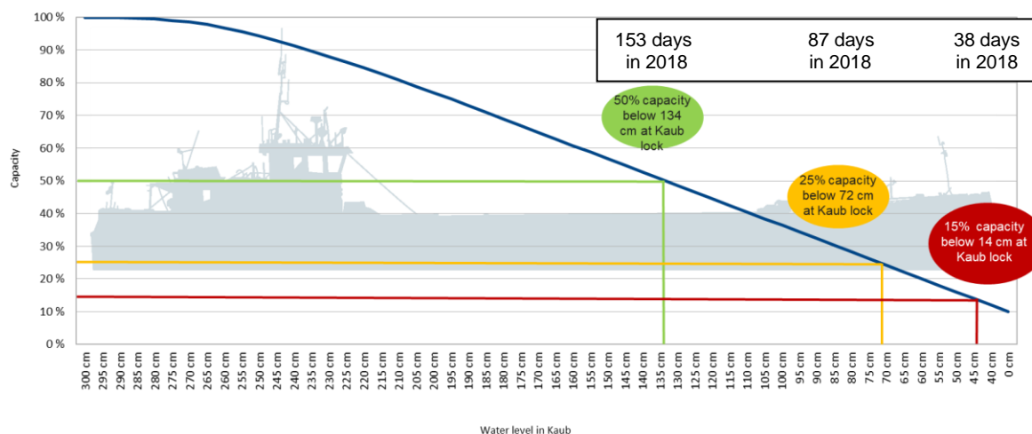
Figure 18: Fleet capacity vs water levels at Kaub (Source: Rhemus Logistics)
