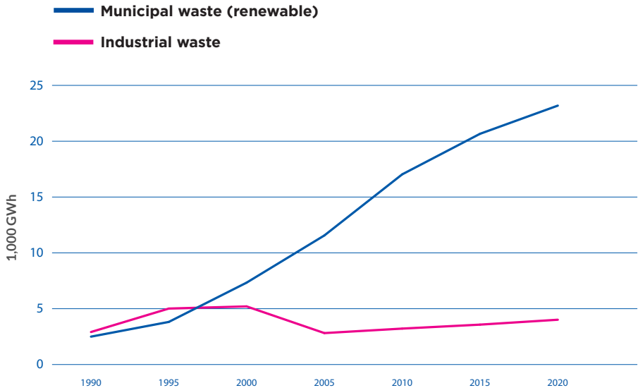
FIG. 1: ELECTRICITY GENERATION FROM WASTE IN THE EUROPEAN UNION 28 (1,000 GWh)
