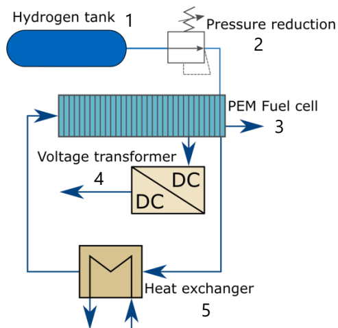
Figure 30: General schema of the Hydrogen system
