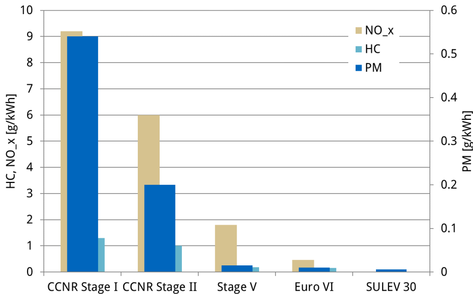
Figure 18: Emission limits for Stage I to Stage V for HC, NO x and PM [26]
