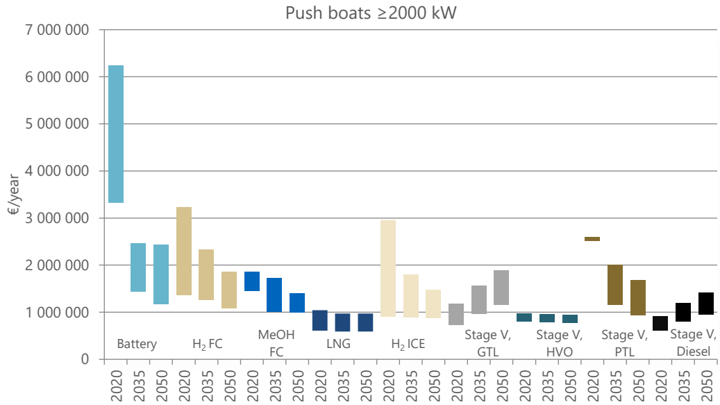
Figure 39: TCO for the type ship of the fleet family push boats with a main propulsion power of more than 2,000 kW
