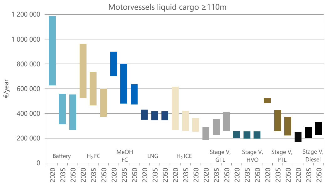
Figure 40: TCO for the type ship of the fleet family motorvessels with liquid cargo \geq 110 m
